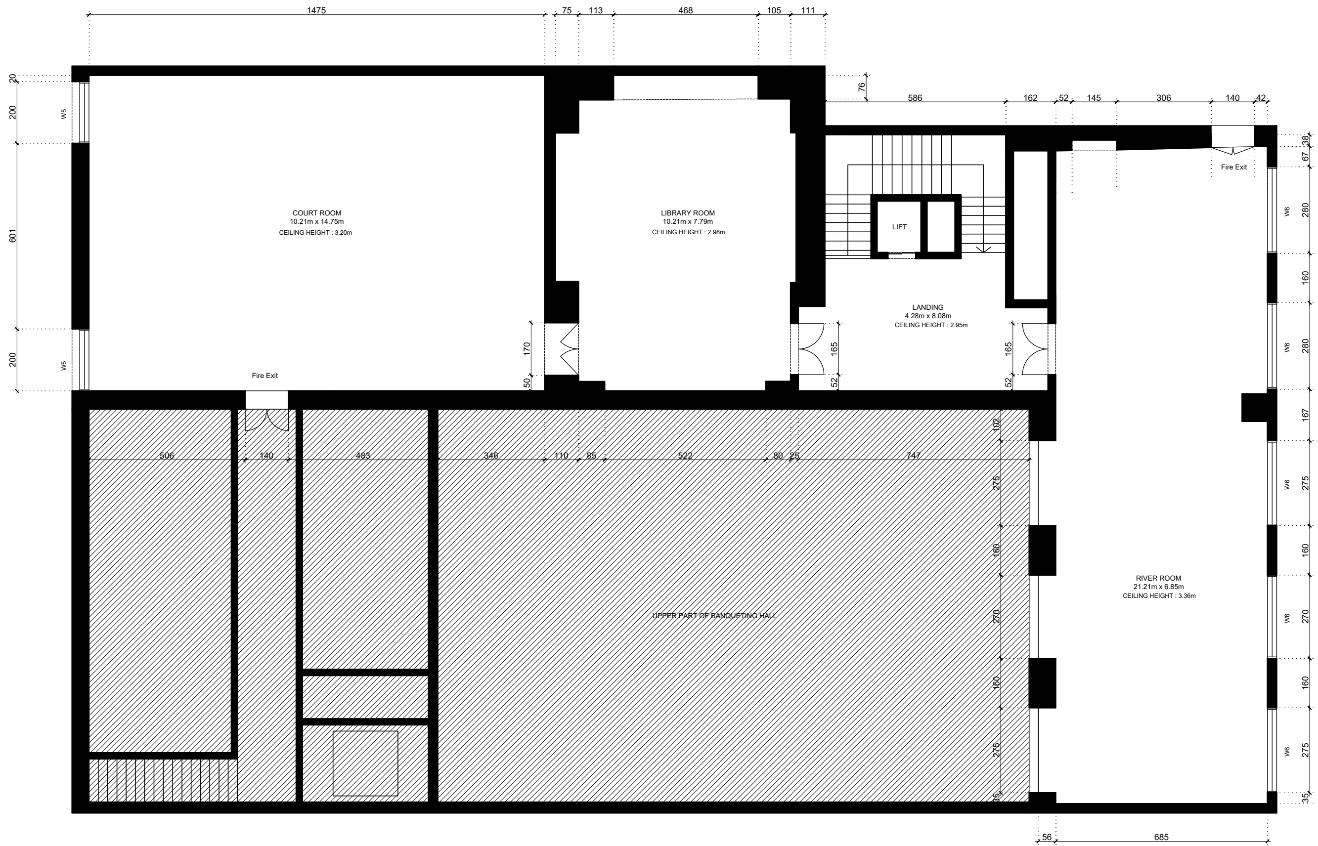
GLAZIERS HALL, FIRST FLOOR PLAN, 450.17 M 2
